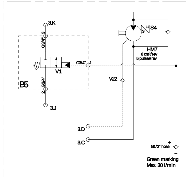
Central Seed Fill 2,2m3 (Option)
